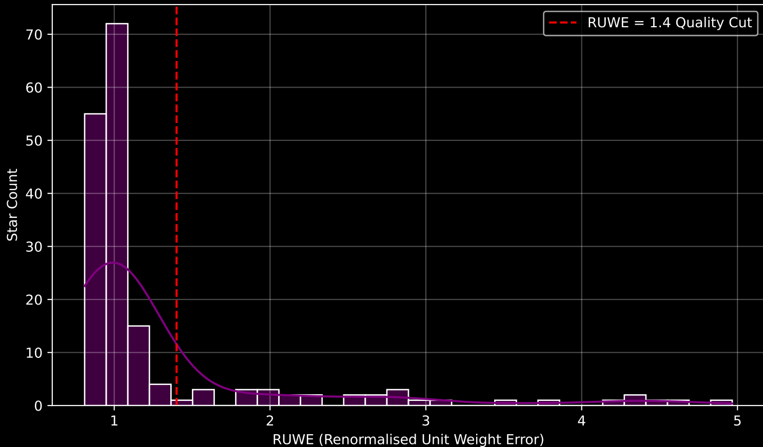
GAPOGEE DR17 Field [102+61_MGA] RUWE Distribution (n= 177)
