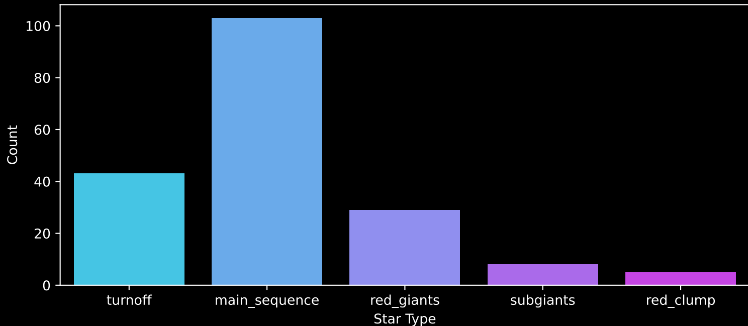
APOGEE DR17 Field: [102+61_MGA] Count plot of Star Type
