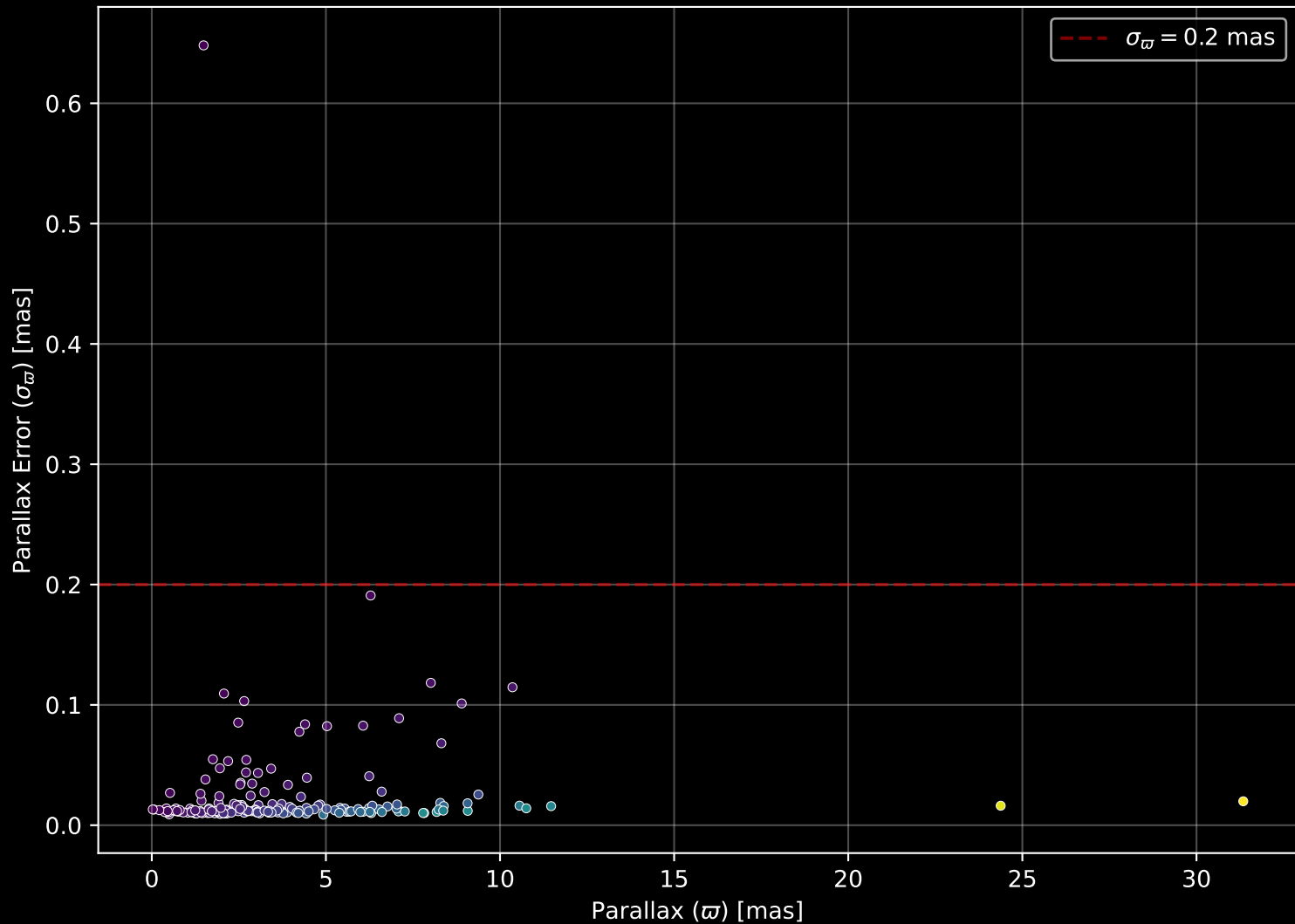
APOGEE DR17 Field: [102+61_MGA] Parallax Quality (n= 188)
