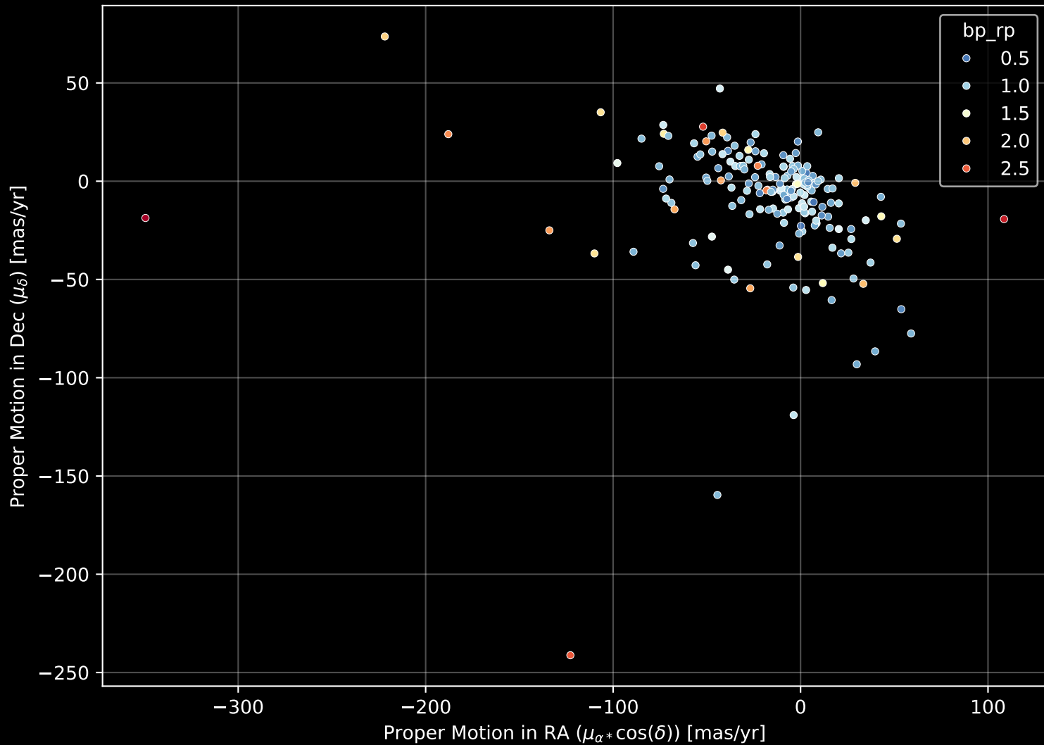
APOGEE DR17 Field: [102+61_MGA] Proper Motion Diagram (n= 188)
