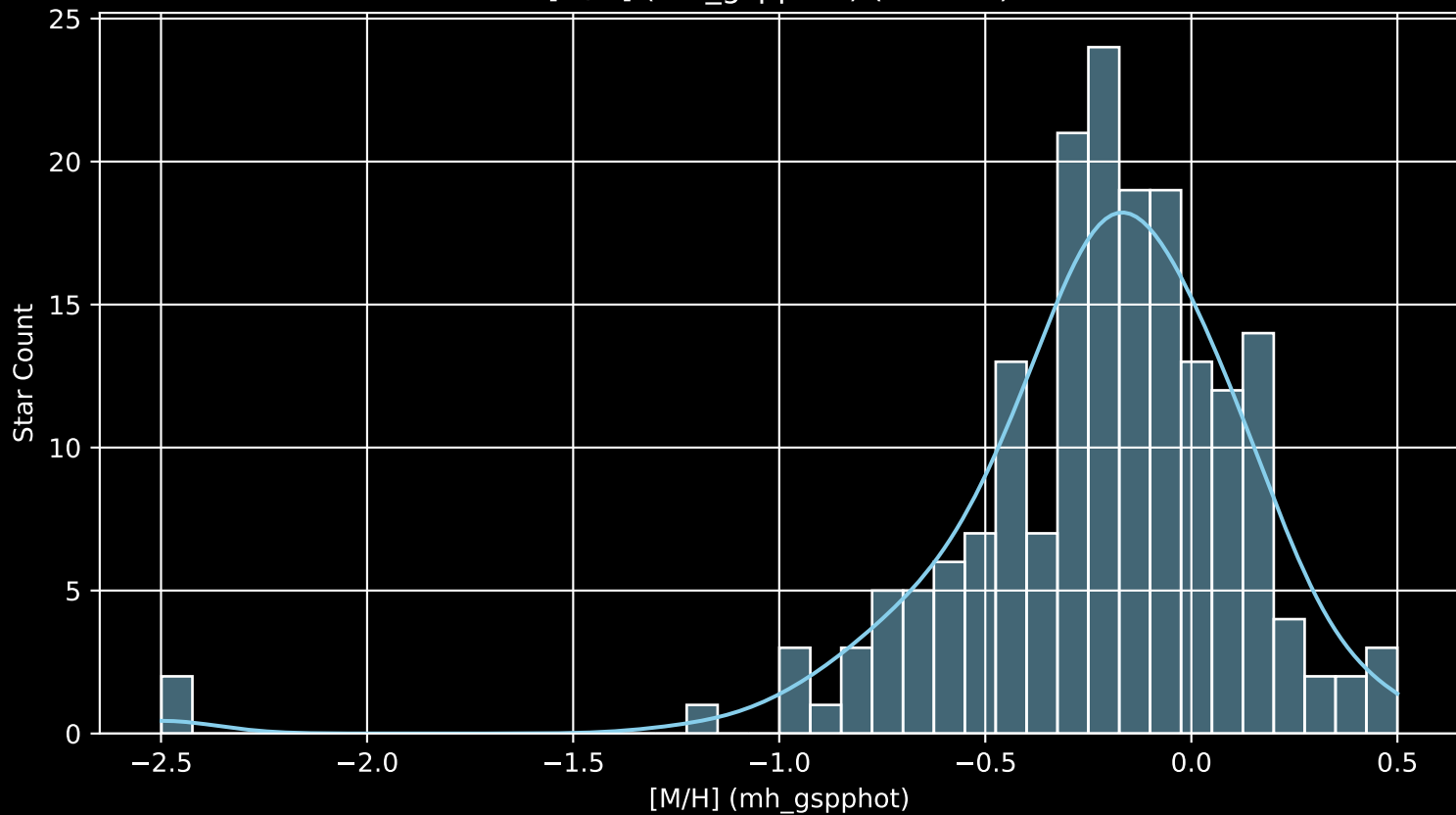
APOGEE DR17 Field: [102+61_MGA [M/H] (mh_gspphot) (n= 186)
