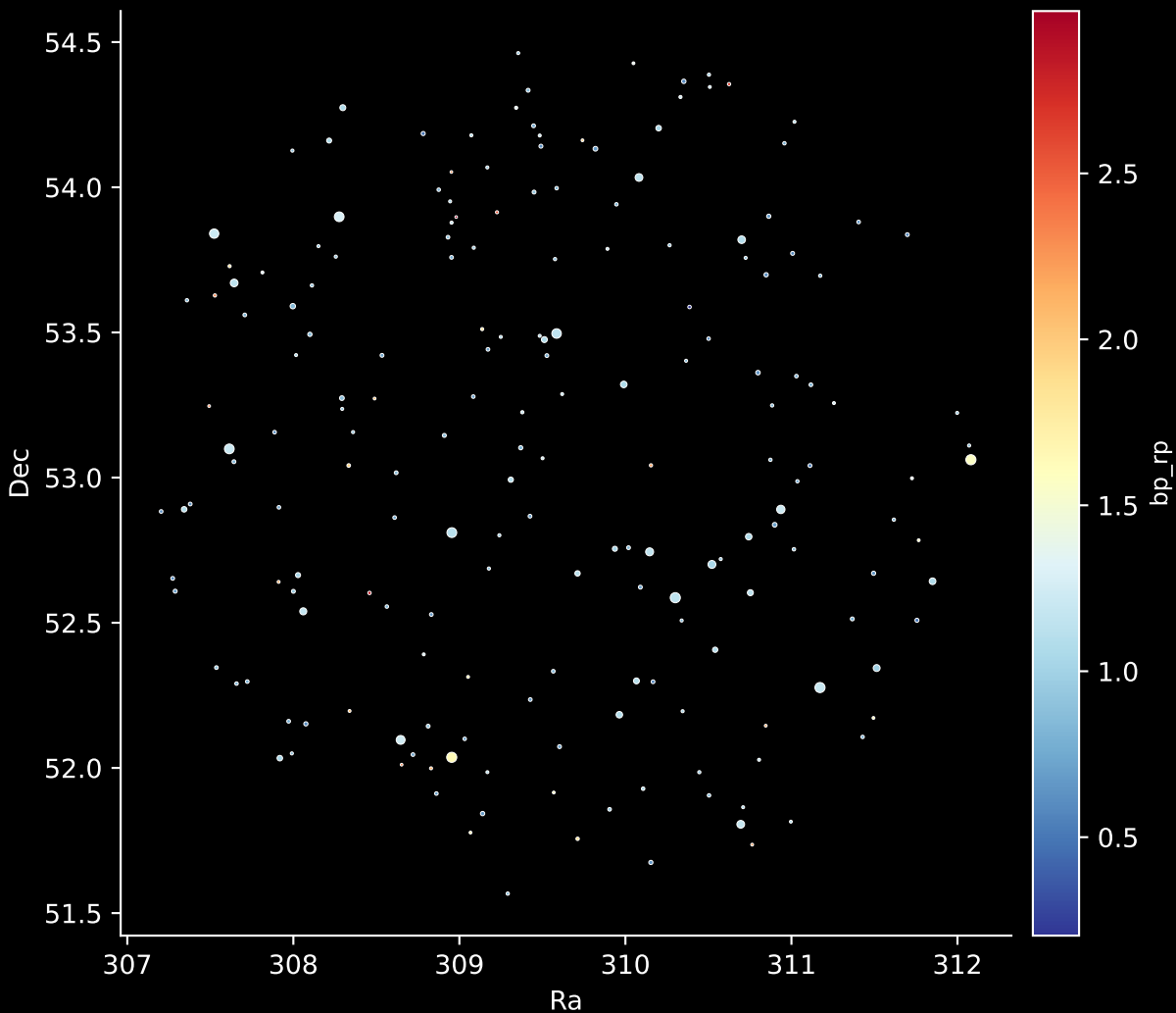
APOGEE DR17 Field: [102+61_MGA] Stars: 188
